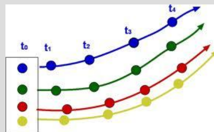
Pathlines
